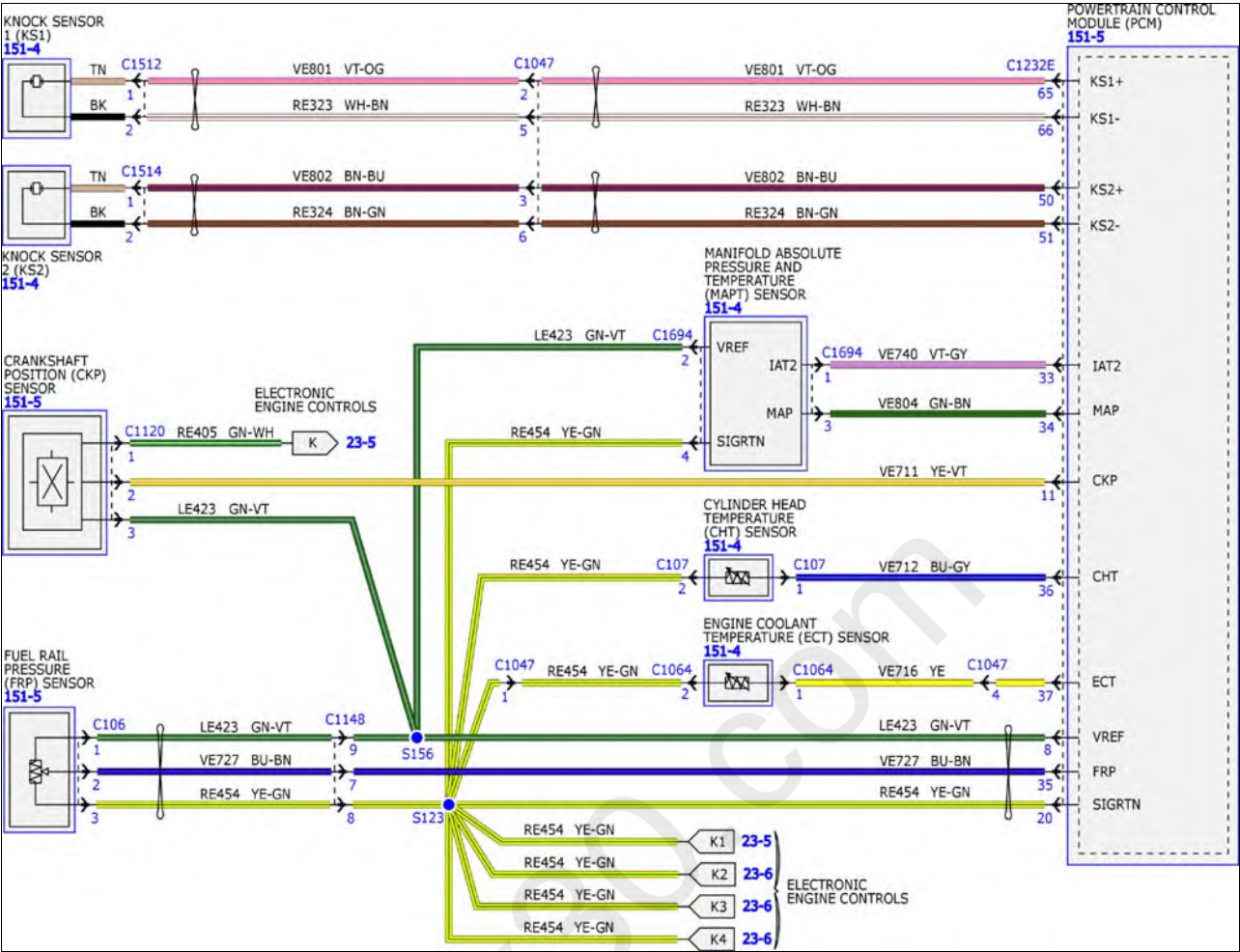
Fig 9: Electronic Engine Controls System Wiring Diagrams (9 Of 15) - 2.7L
