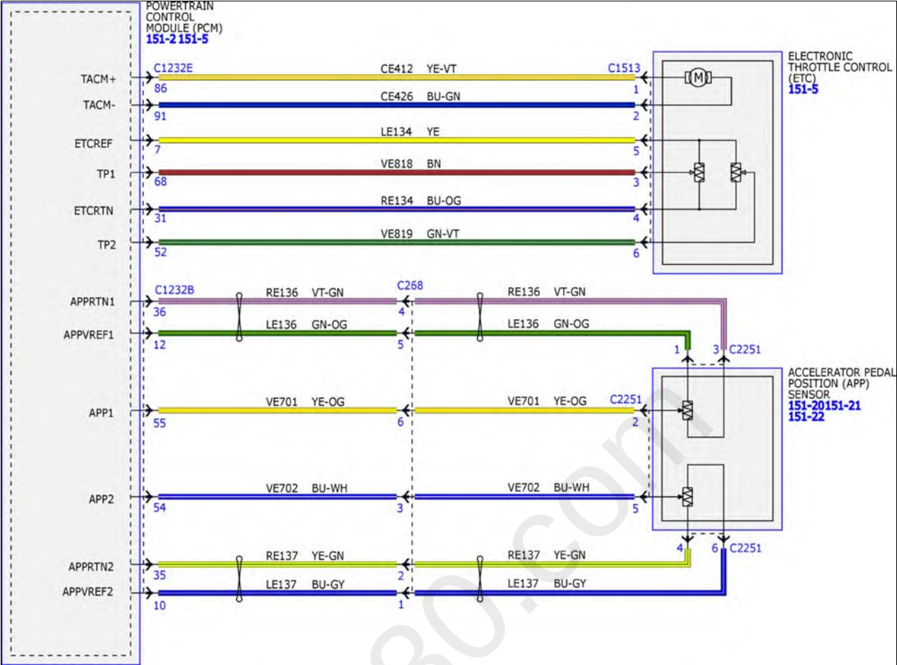
Fig 3: Electronic Engine Controls System Wiring Diagrams (3 Of 15) - 2.7L
