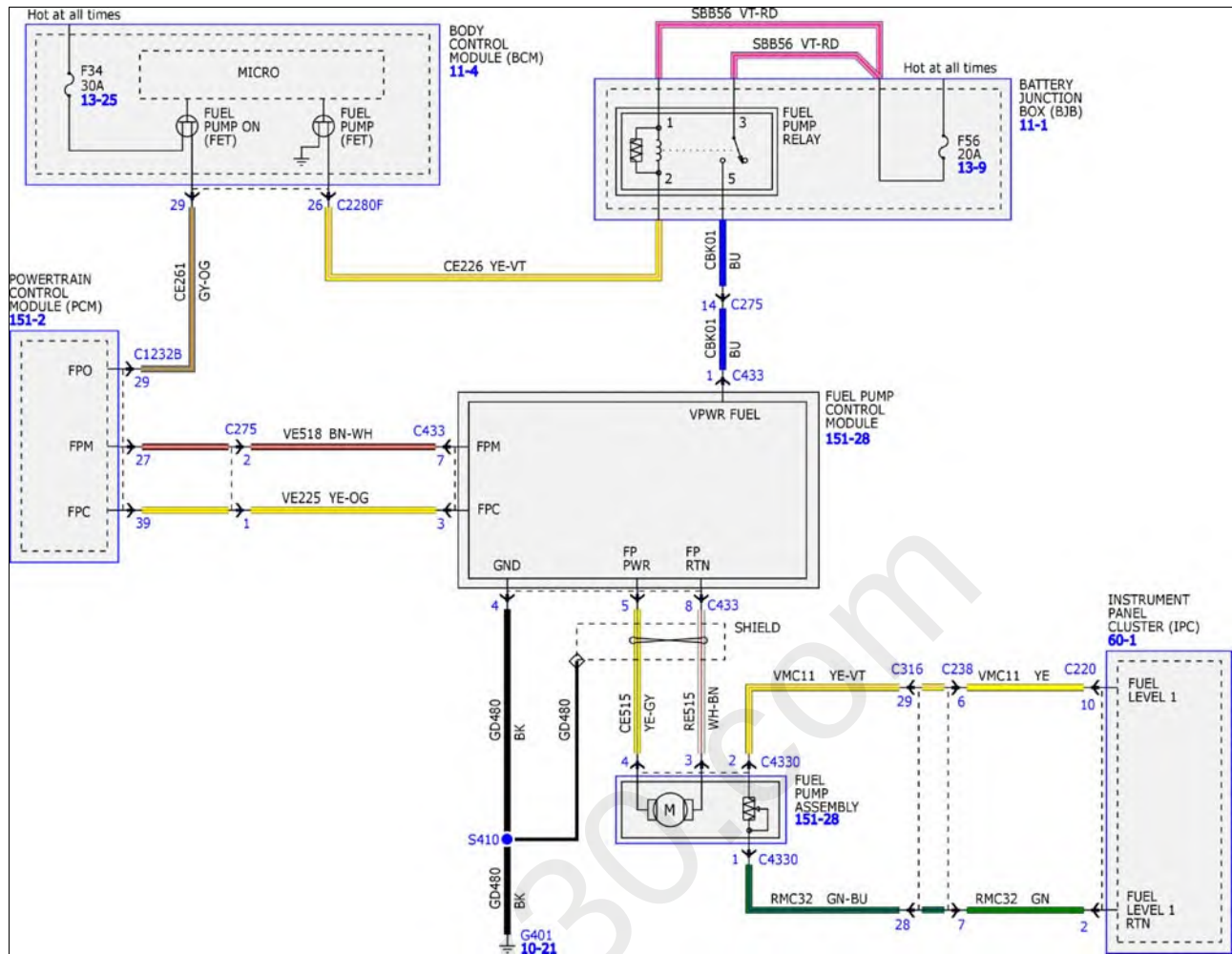
Fig 4: Electronic Engine Controls System Wiring Diagrams (4 Of 15) - 2.7L
