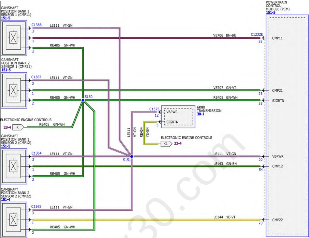
Fig 10: Electronic Engine Controls System Wiring Diagrams (10 Of 15) - 2.7L
