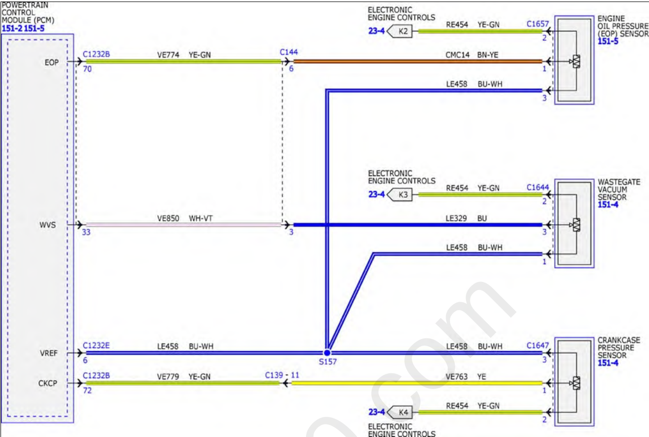
Fig 11: Electronic Engine Controls System Wiring Diagrams (11 Of 15) - 2.7L
