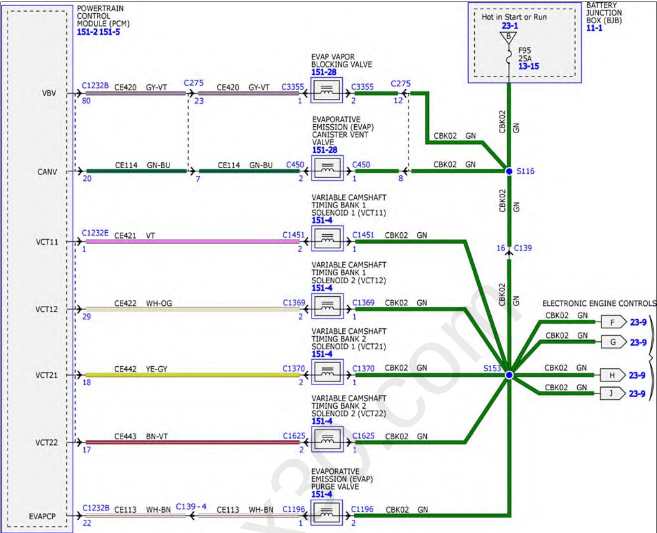
Fig 13: Electronic Engine Controls System Wiring Diagrams (13 Of 15) - 2.7L
