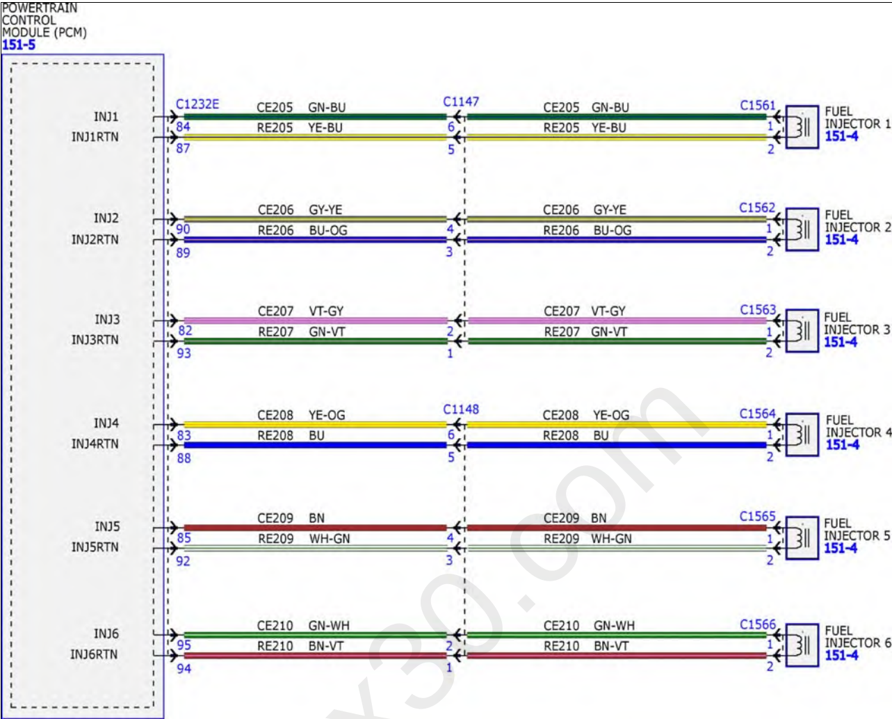
Fig 8: Electronic Engine Controls System Wiring Diagrams (8 Of 15) - 2.7L
