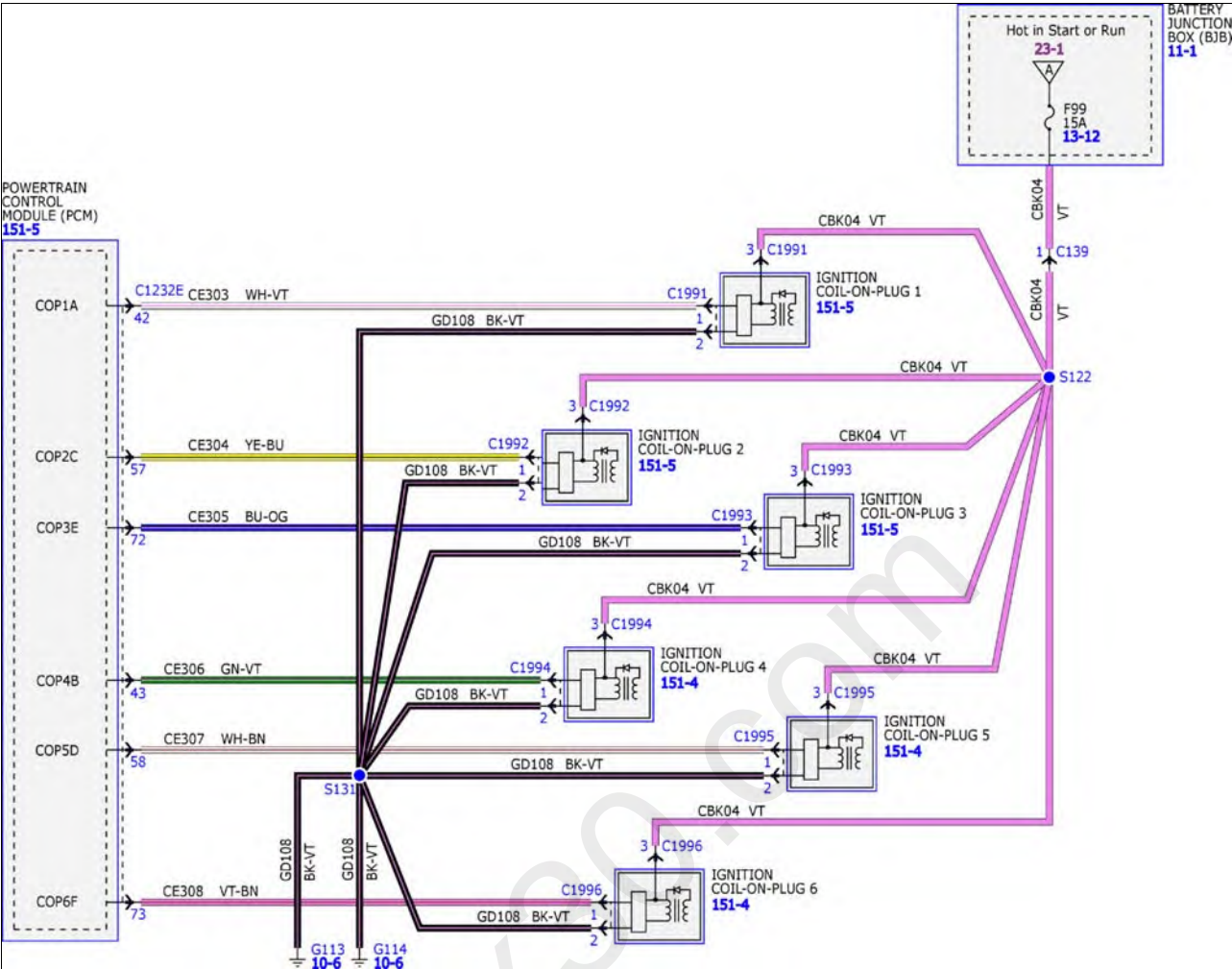
Fig 2: Electronic Engine Controls System Wiring Diagrams (2 Of 15) - 2.7L
