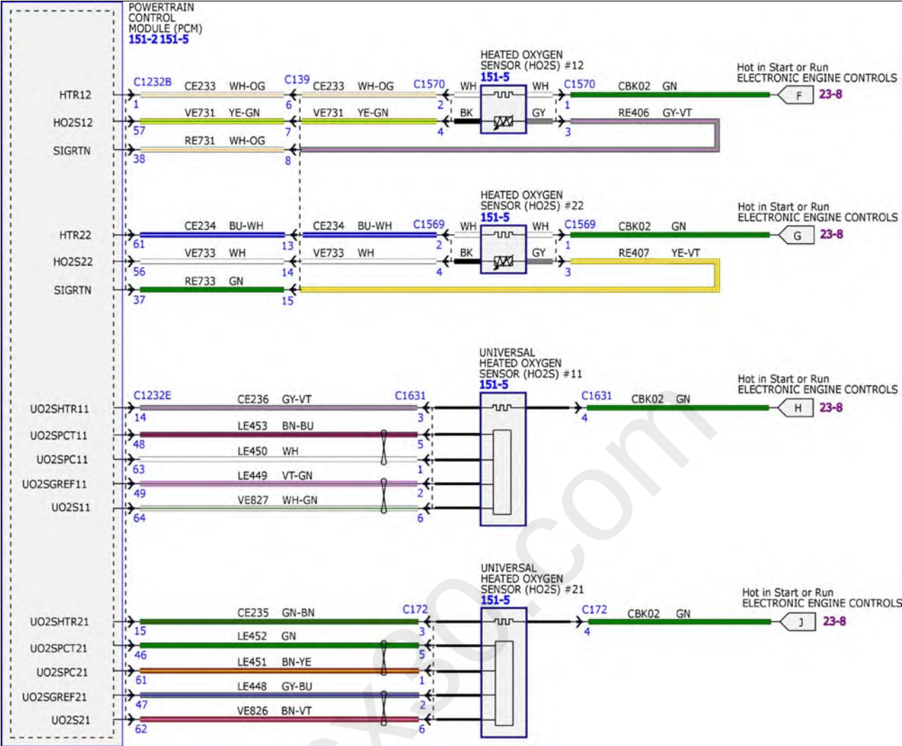
Fig 14: Electronic Engine Controls System Wiring Diagrams (14 Of 15) - 2.7L
