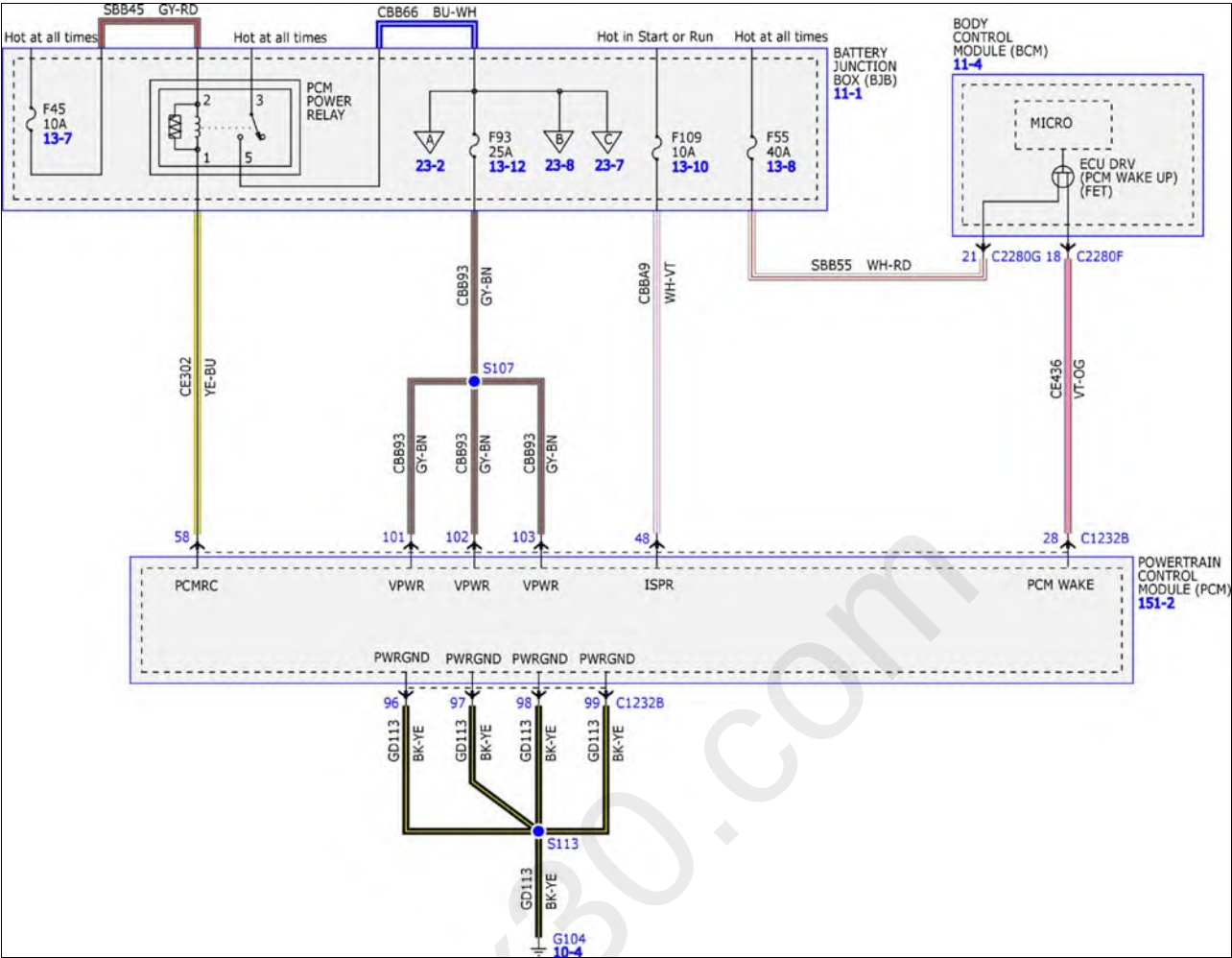
Fig 1: Electronic Engine Controls System Wiring Diagrams (1 Of 15) - 2.7L
