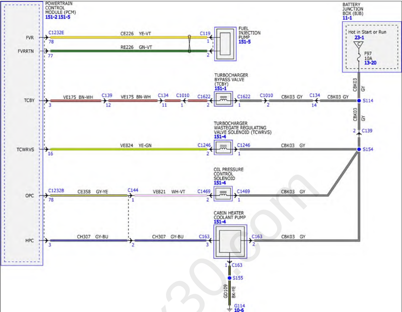
Fig 12: Electronic Engine Controls System Wiring Diagrams (12 Of 15) - 2.7L
