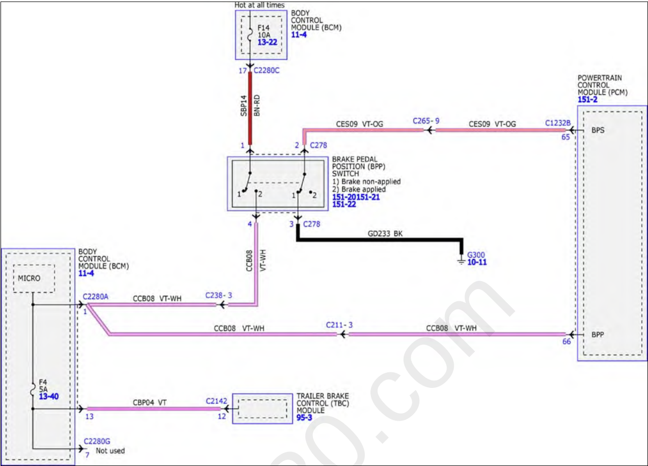
Fig 6: Electronic Engine Controls System Wiring Diagrams (6 Of 15) - 2.7L
