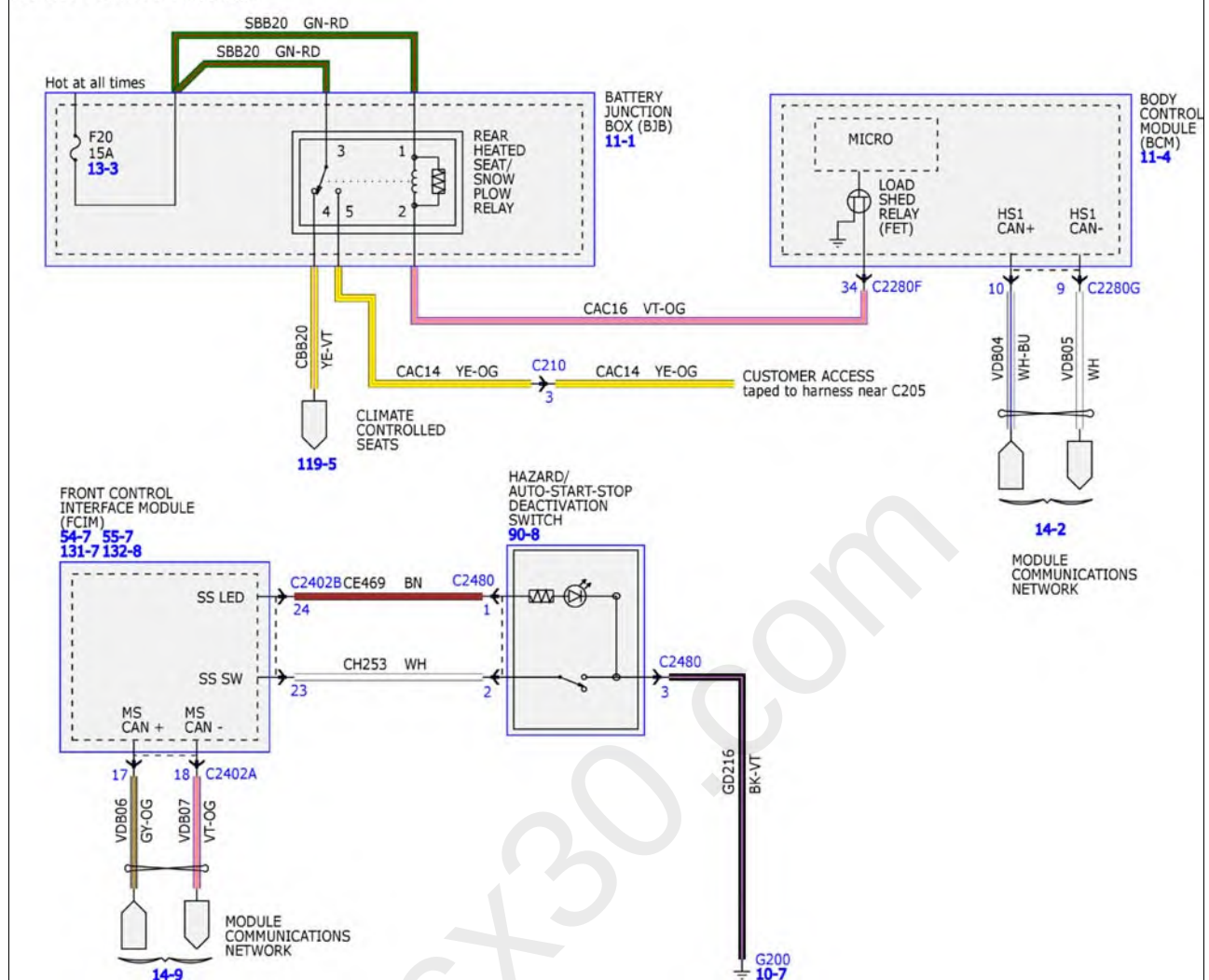
Fig 1: Customer Access System Wiring Diagram
