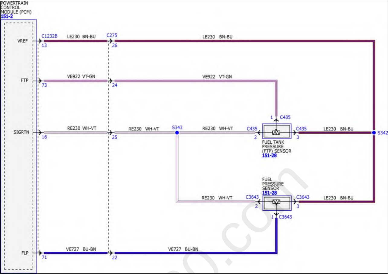
Fig 5: Electronic Engine Controls System Wiring Diagrams (5 Of 15) - 2.7L
