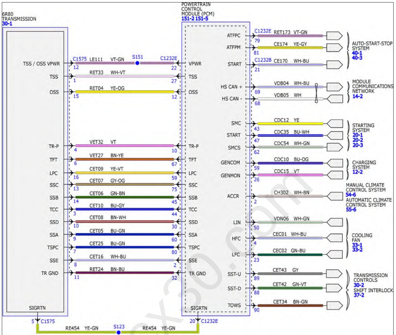
Fig 7: Electronic Engine Controls System Wiring Diagrams (7 Of 15) - 2.7L
